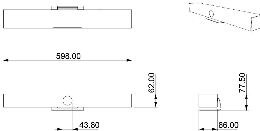
Figure 2.1 Dimensions
