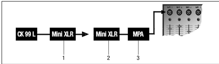
Fig. 1: Connection diagram with optional MPA V L
